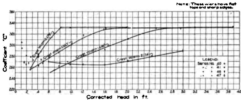
FIG. 16.—Experiments on flow over broad-crested weirs Cornell University Hydraulic Laboratory, 1903. (U. S. Geological Survey—Water-Supply Paper No. 200.)
